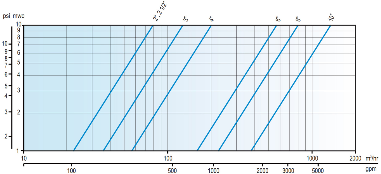
OCV Model 68 Head Loss
